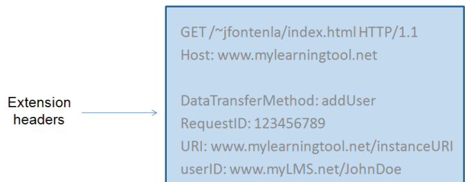
Figure 4. Sample message of the Instance Protocol.
